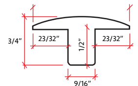
T-Molding 78" in Length
