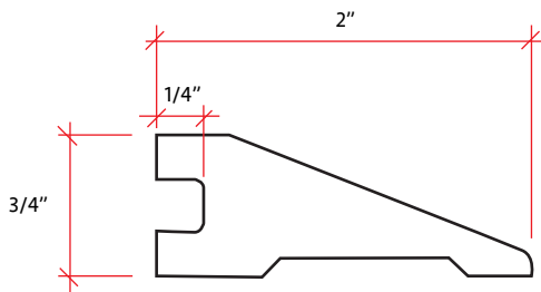
Reducer 78" in Length
