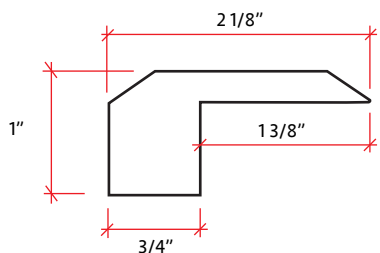
Threshold 78" in Length
