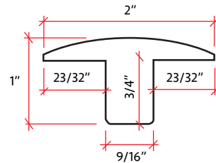
T-Molding 78" in Length
