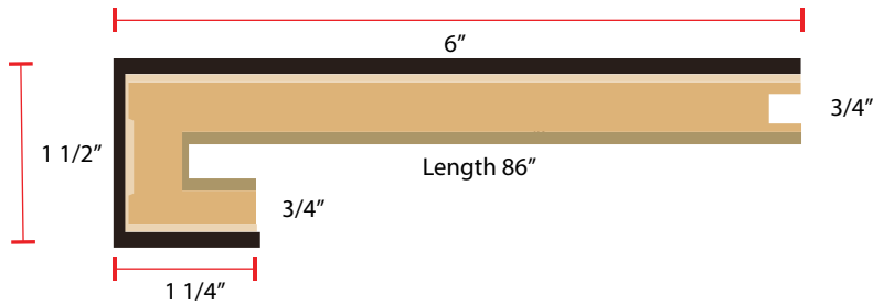
Fabricated Stair Nose
