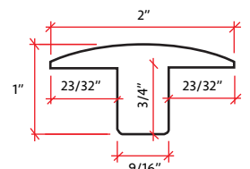
T-Molding 78" in Length
