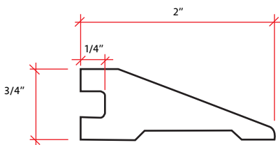
Reducer 78" in Length
