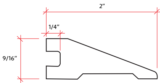
Reducer 78" in Length
