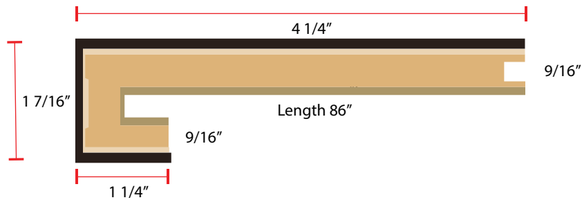
Fabricated Stair Nose
